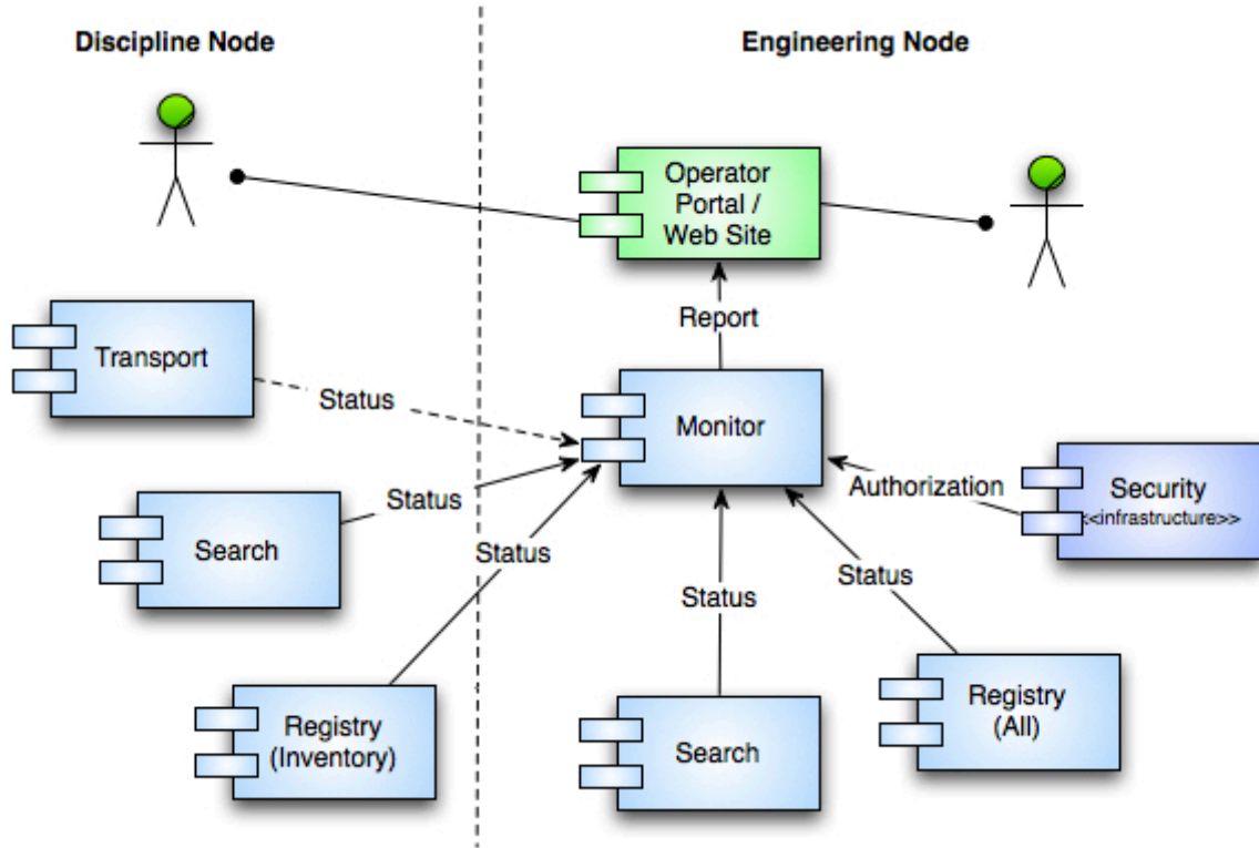
Figure 11.9: Monitoring Scenario
