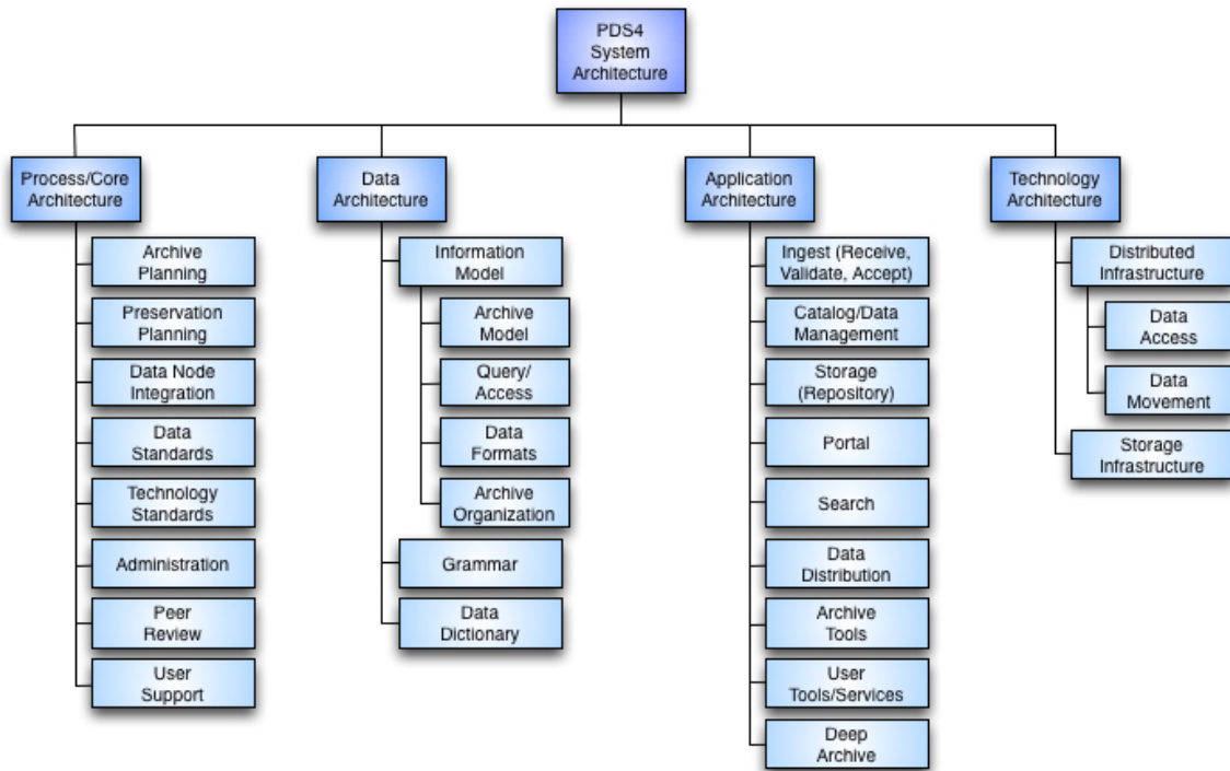
Figure 8.1: Architectural Decomposition
