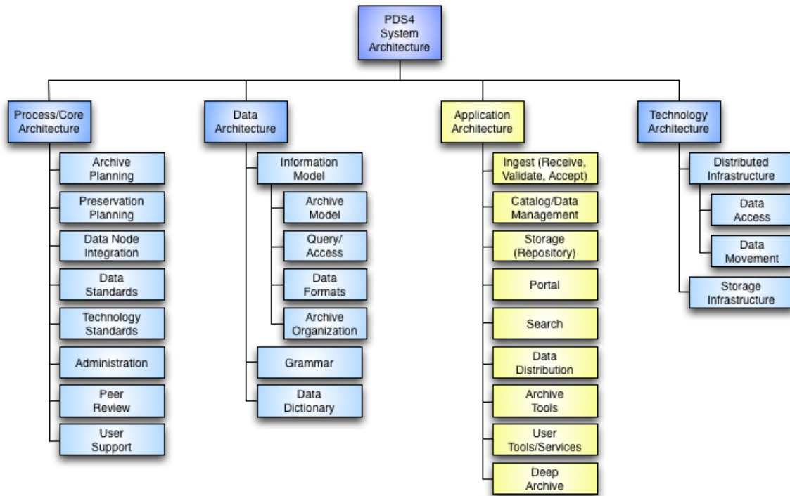
Figure 11.1: Architectural Decomposition
