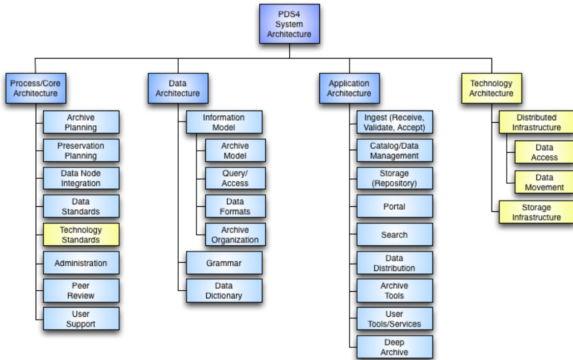
Figure 12.1: Architectural Decomposition
