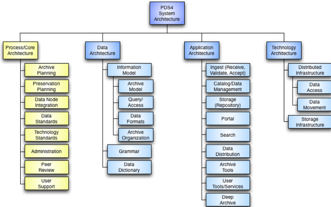
Figure 9.1: Architectural Decomposition
