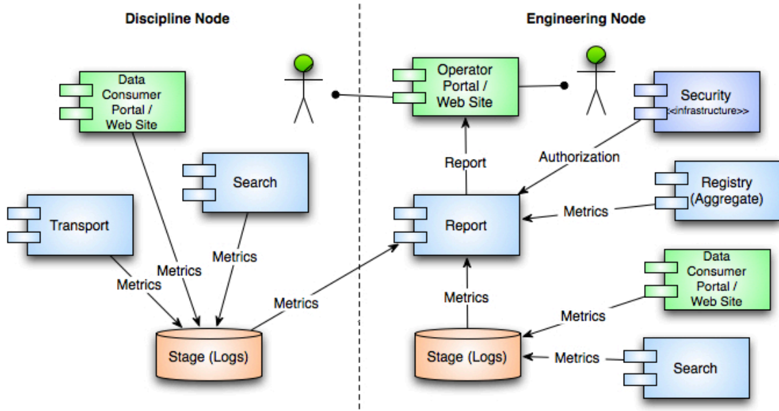
Figure 11.10: Reporting Scenario
