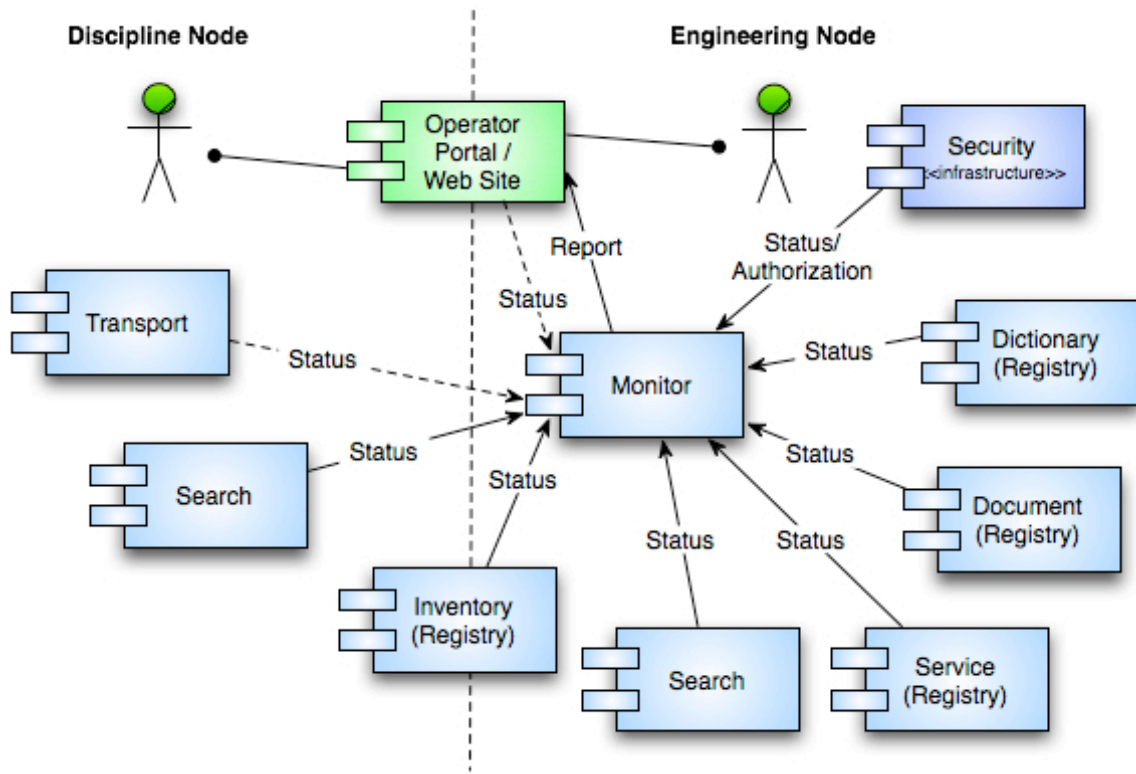
Figure 11.9: Monitoring Scenario
