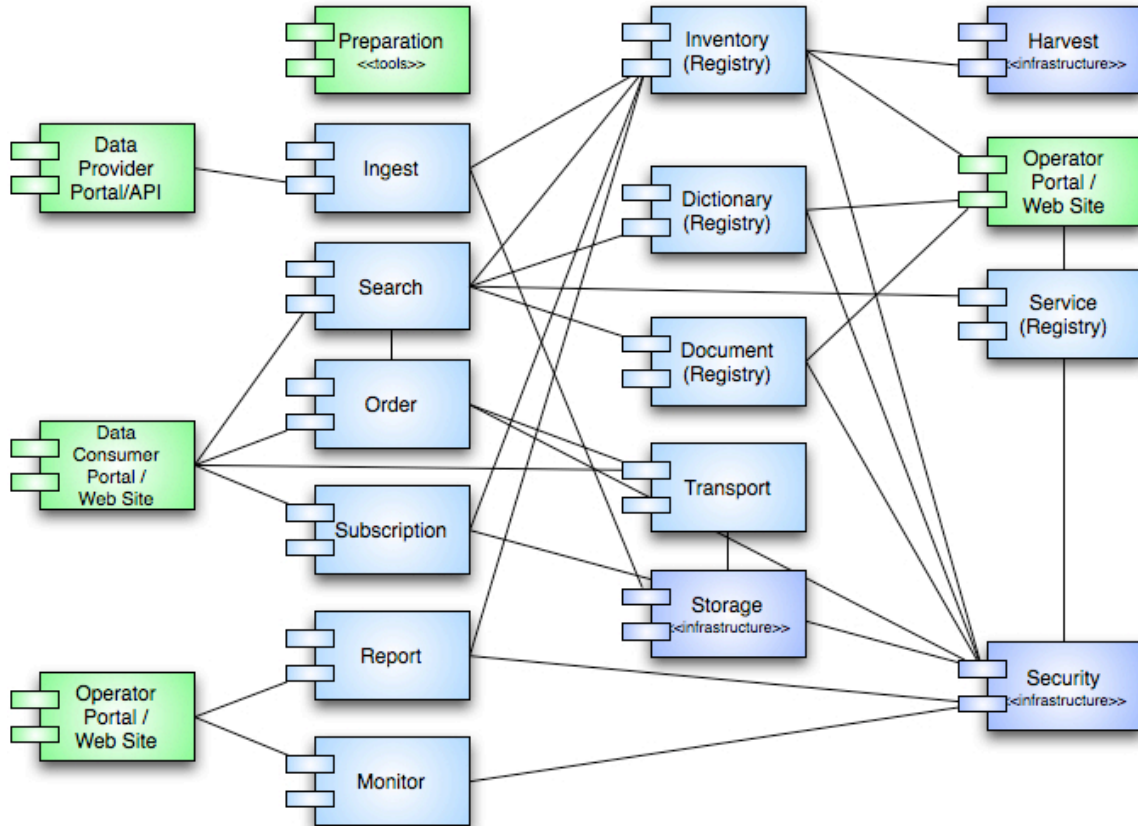
Figure 11.2: System Context
